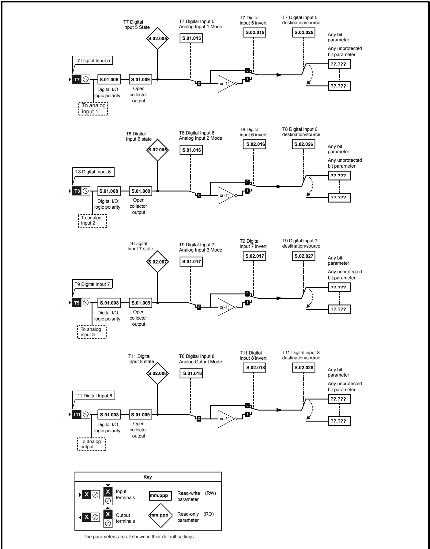
Figure 8-3 Digital input 5/6/7/8
